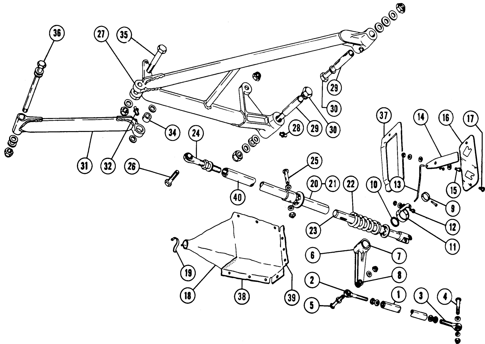
Figure 56. Nose Gear Retract Assembly
